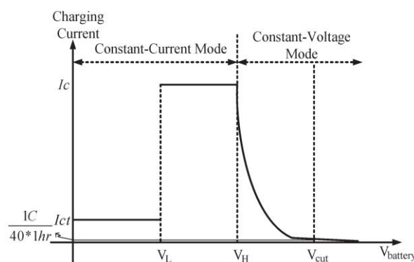
Figure 1. Three modes of battery charging, CC/CV algorithm [17]
